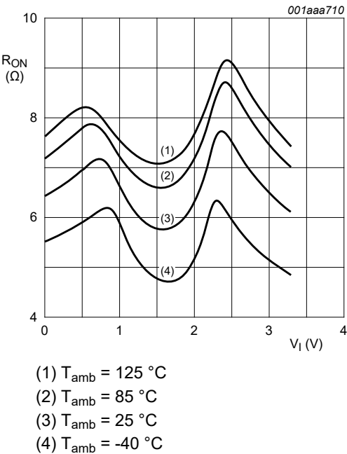
Fig. 15. ON resistance as a function of input voltage; V_{CC} = 3.3\text{ V}
