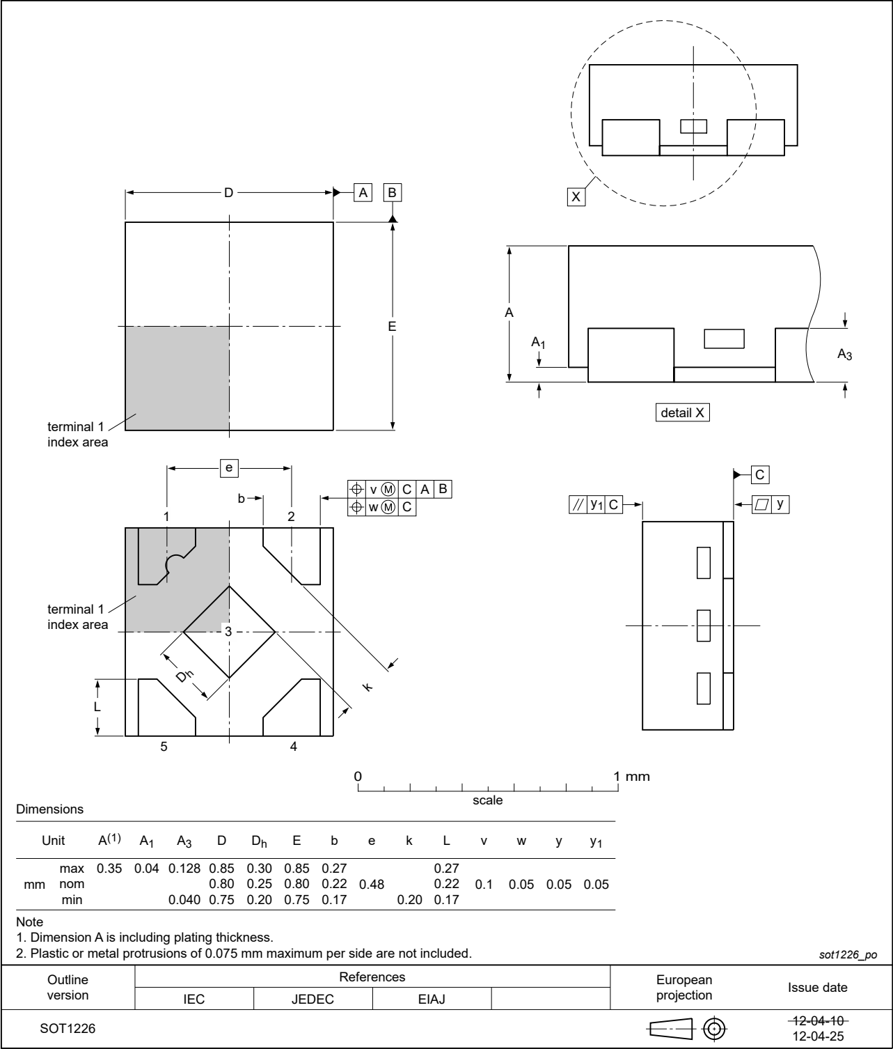
Fig. 30. Package outline SOT1226 (X2SON5)
