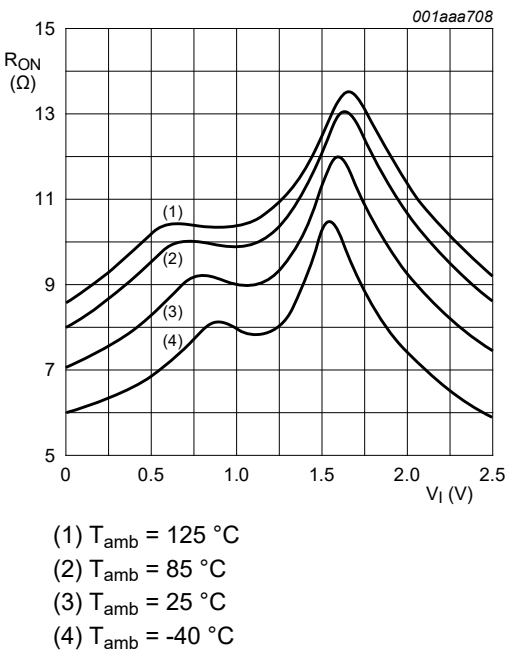
Fig. 13. ON resistance as a function of input voltage; V_{CC} = 2.5\text{ V}
