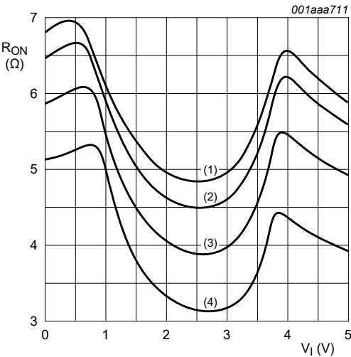
Fig. 14. ON resistance as a function of input voltage; V_{CC} = 2.7\text{ V}
